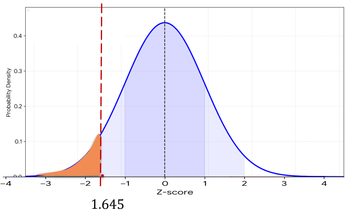
Z-table (Standard Normal Distribution Table).
